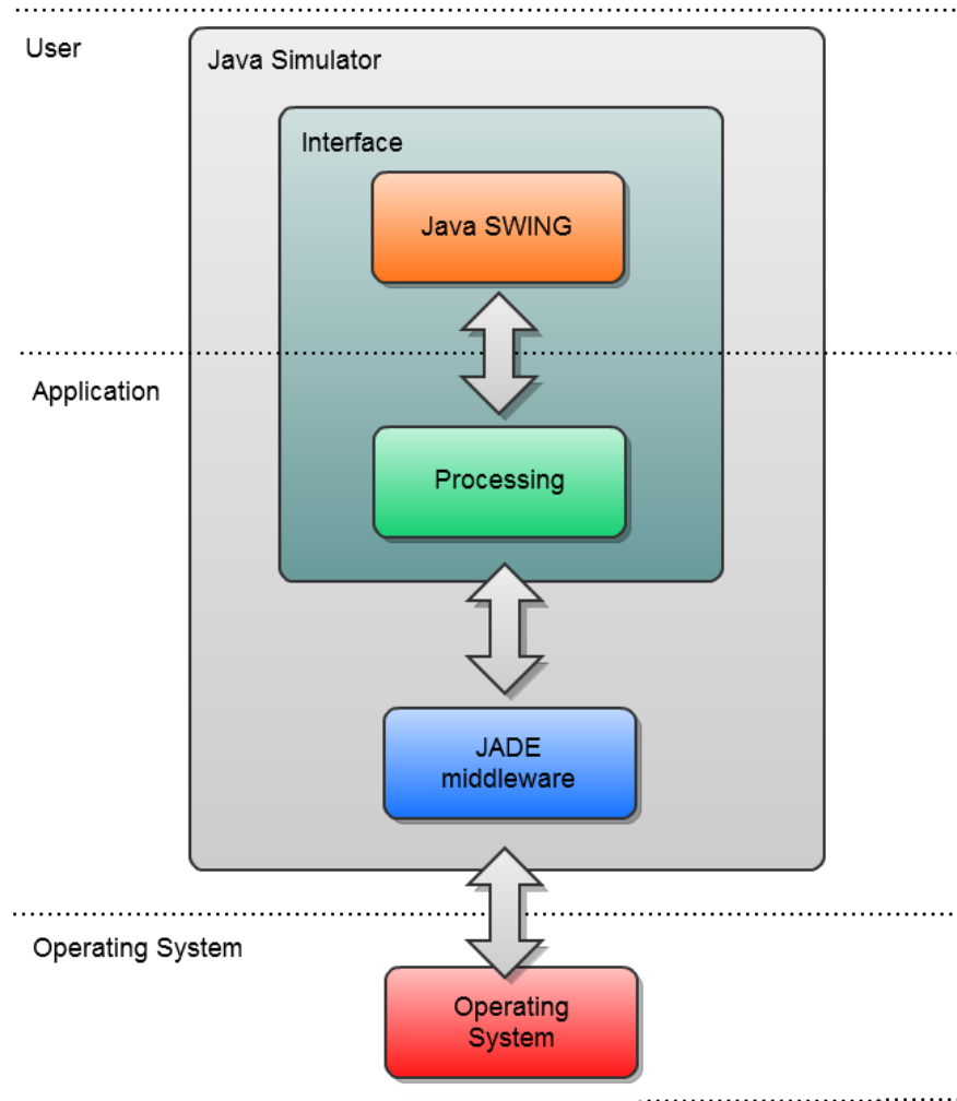
Figure 5.3: Logical Architecture
