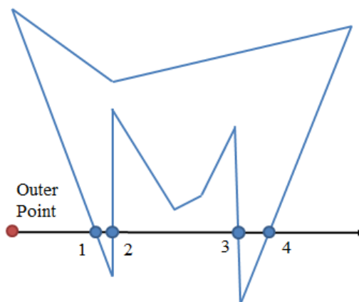
Figure 4.8: Ray Casting
