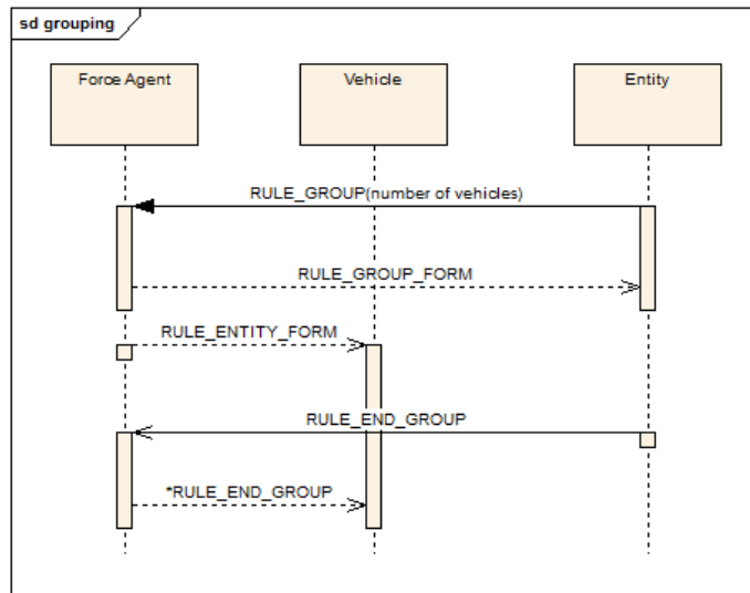
Figure 4.13: Grouping communication
