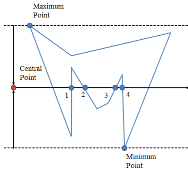
Figure 4.9: Ray Casting Implementation
