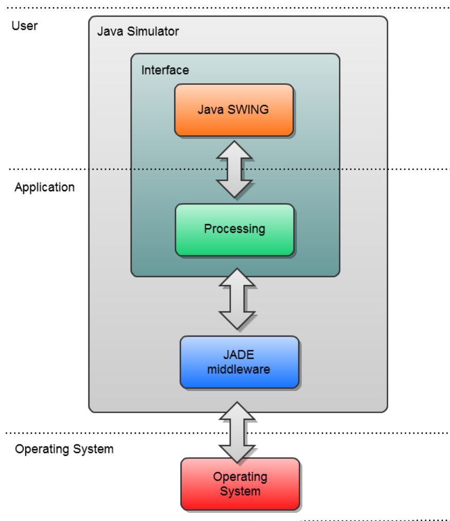
Figure 4.3: Logical Architecture
