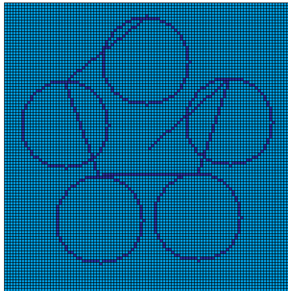
Figure 4.5: Survey Behavior
