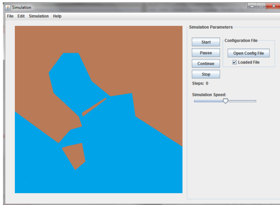
Figure 4.10: Simulator's Interface
