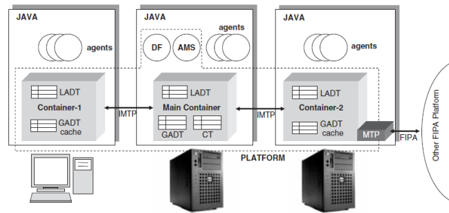
Figure 4.1: JADE architecture [Bel07]
