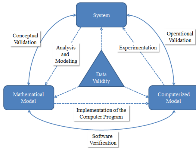
Figure 2.2: Verification, Validation and Accreditation Diagram [Sar91]
