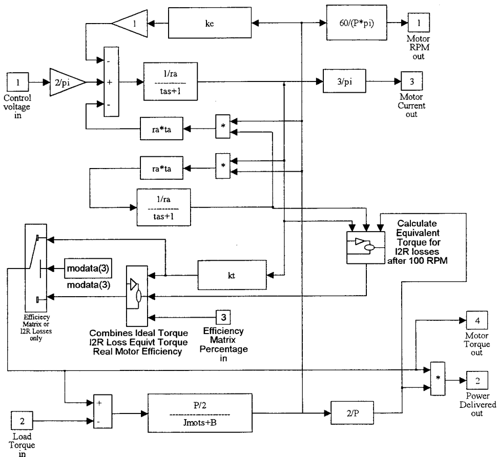
Figure 3-3. PMDC Motor Block
