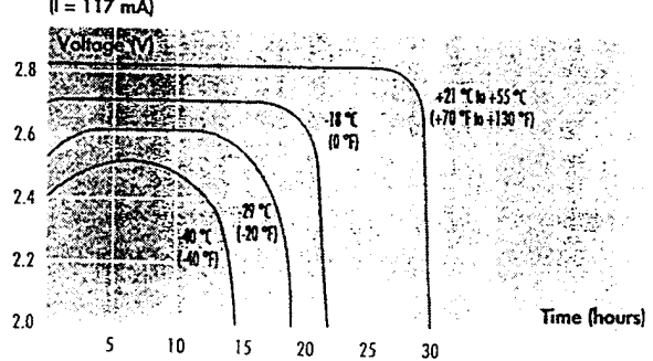
LO40 SHX - Discharge profiles (I = 117 mA)
