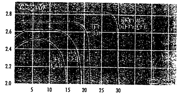
LO26 SX - Discharge profiles
