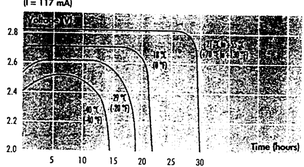
LO29 SHX - Discharge profiles (I = 117 mA)
