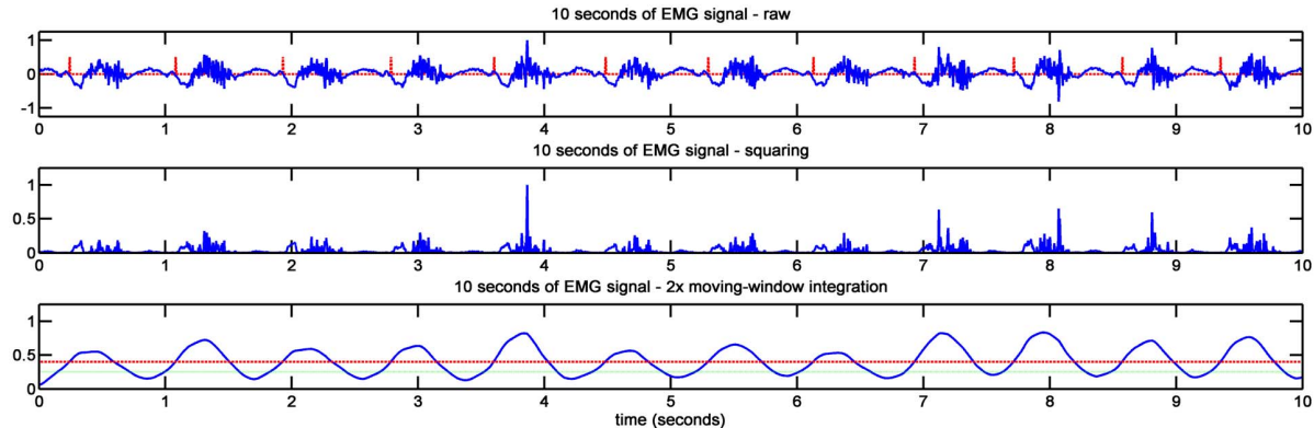
Figure 2. Processing pipeline for the EMG signal. In this figure, 10 seconds of the signal were extracted for the processing. From top to bottom: (1) raw EMG signal ( blue, solid ), detected treads by the algorithm ( red, dashed ); (2) signal after squaring operation, (3) signal after double moving-window integration ( blue, solid ), threshold ( red, dashed ), minimum threshold for avoiding misdetection ( green, dotted ).
