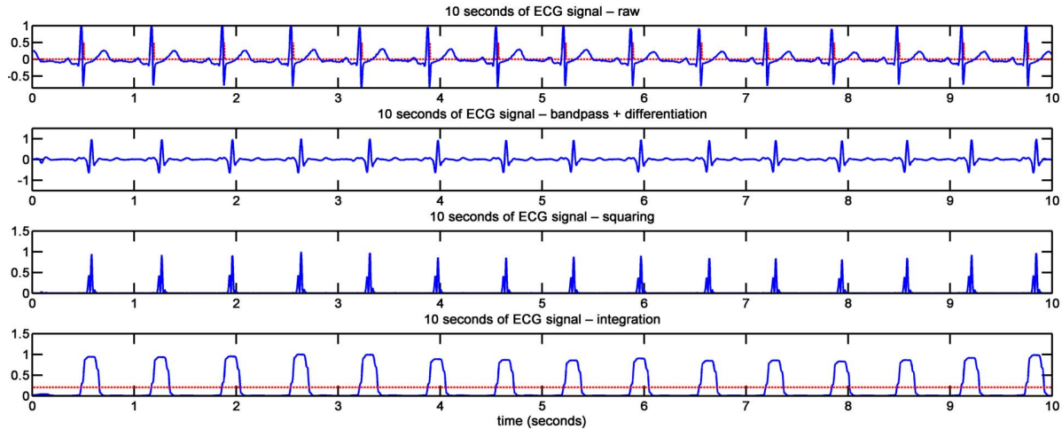
Figure 1. Processing pipeline for the ECG signal. In this figure, 10 seconds of the signal were extracted for the processing. From top to bottom: (1) raw ECG signal ( blue, solid ), detected heart beats by the algorithm ( red, dashed ); (2) signal after bandpass filter and differentiation, (3) signal after squaring operation; (4) signal after moving-window integration ( blue, solid ), threshold ( red, dashed ).
